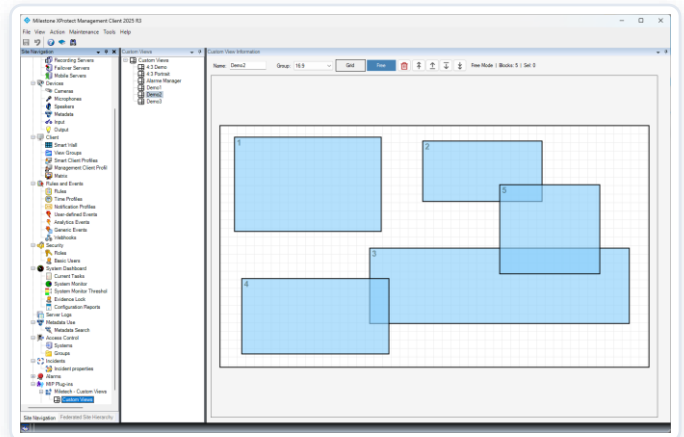
Management Client, free-form layout editor
